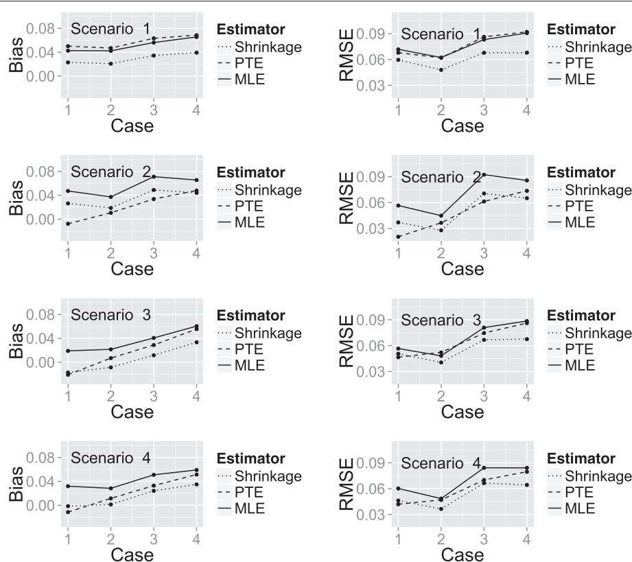
Fig. 4 Plot showing the bias and RMSE of the three estimators. A plot of bias and RMSE for the SHE, PTE and MLE calculated under each true success probability and change in patient status combination
